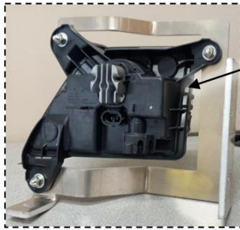
Figure 4a: OEM horizontal fog light installation (driver side shown)
