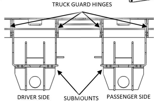
Figure 4c: Submounts position (top view)
