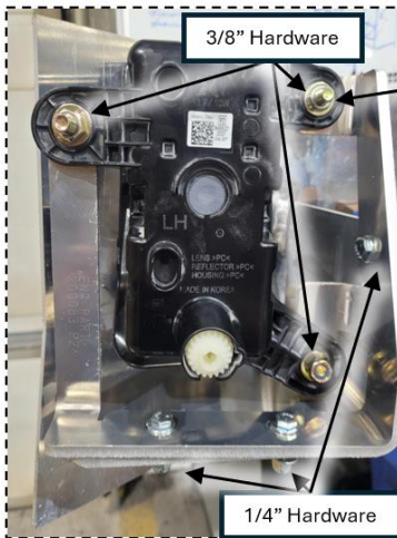
Figure 4e: OEM vertical fog light installation (driver side shown)
