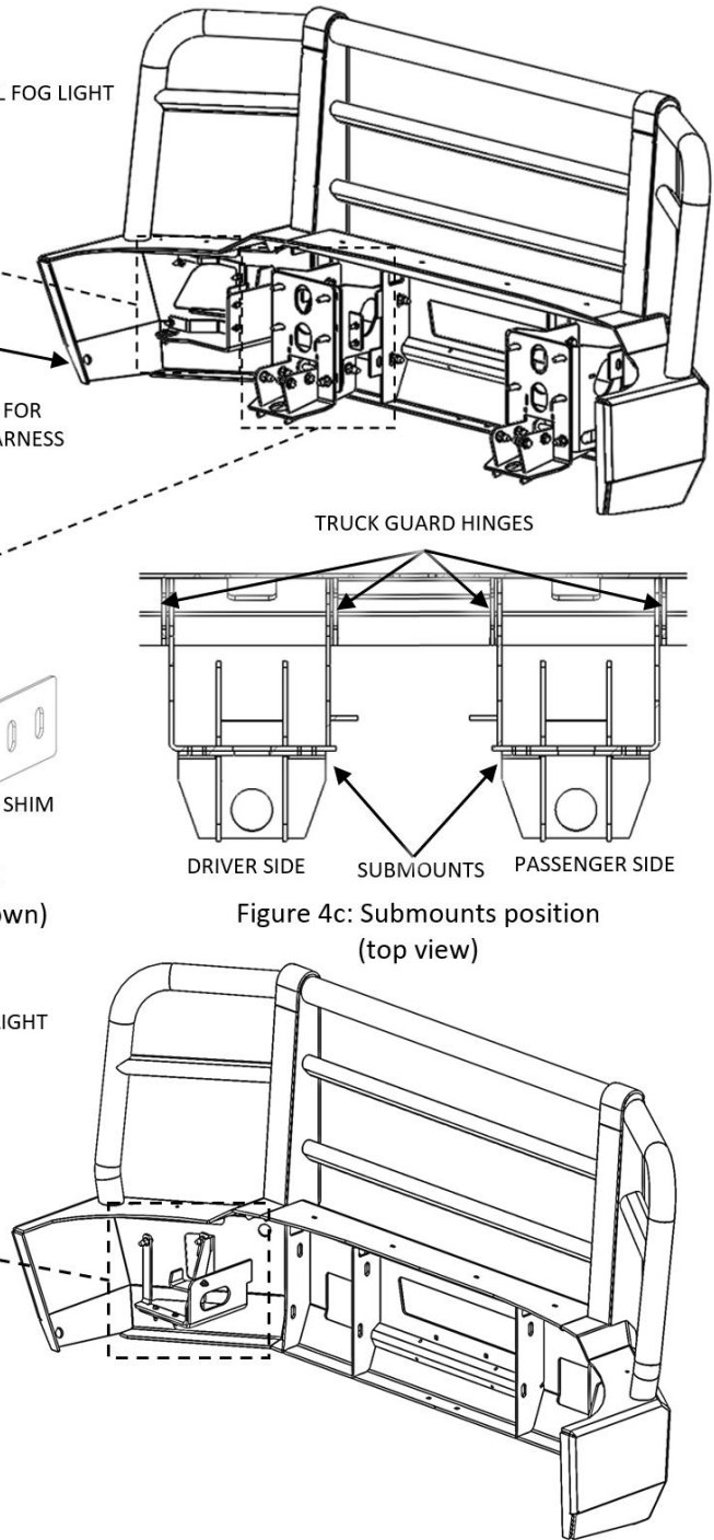
Figure 4: Installing the Truck Guard (view from behind)
