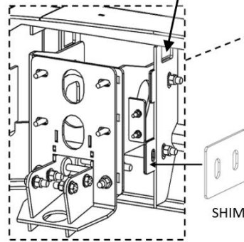
Figure 4b: Truck Guard installation (driver side shown)
