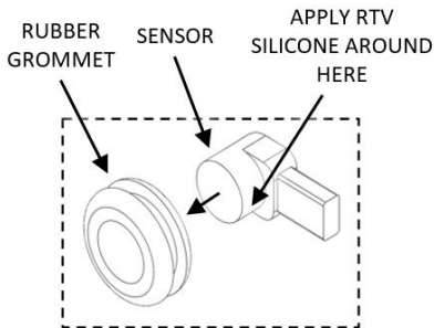
Figure 4d: Sensor installation
